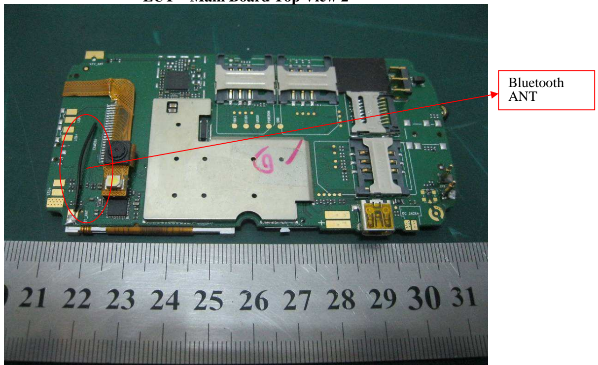
EUT – Main Board Top View 2
