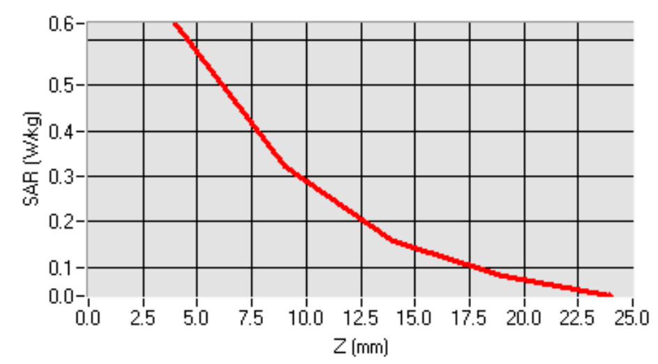
SAR, Z Axis Scan (X = -47, Y = -34)
