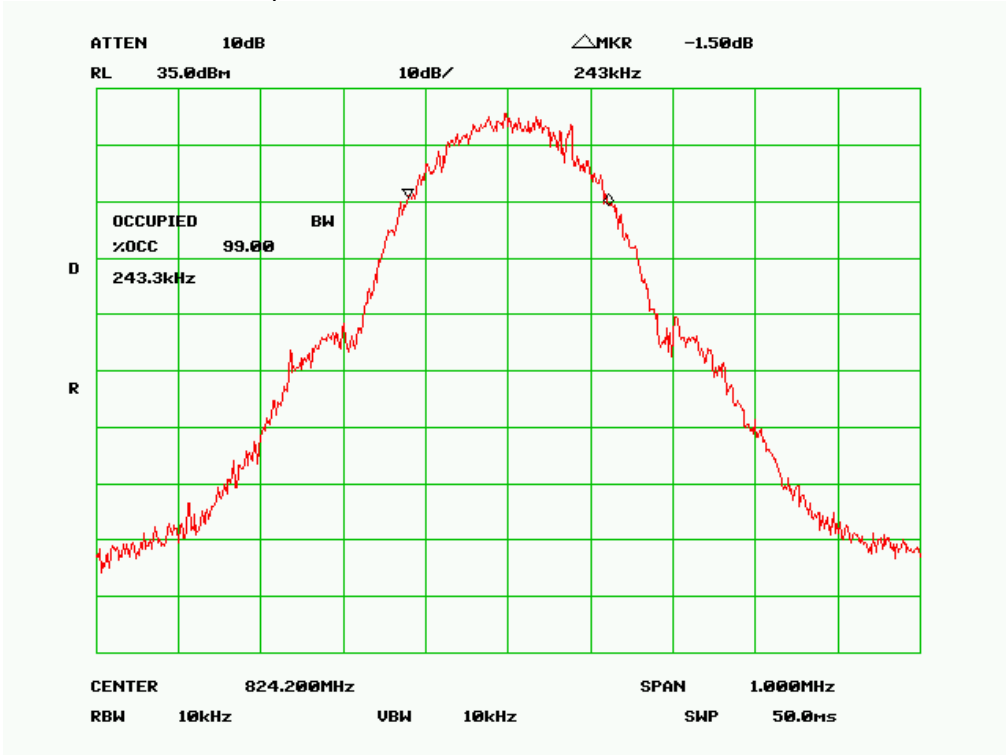
99% Occupied Bandwidth – GPRS850, Channel 128, Low Channel
