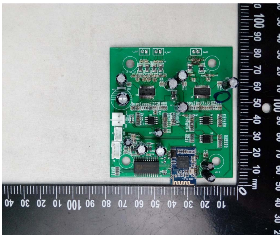
MAIN BOARD 1 FRONT VIEW
