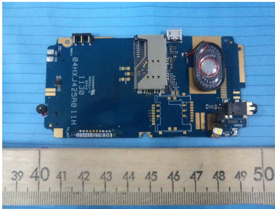
EUT – Mian Board Bottom Shielding off View
