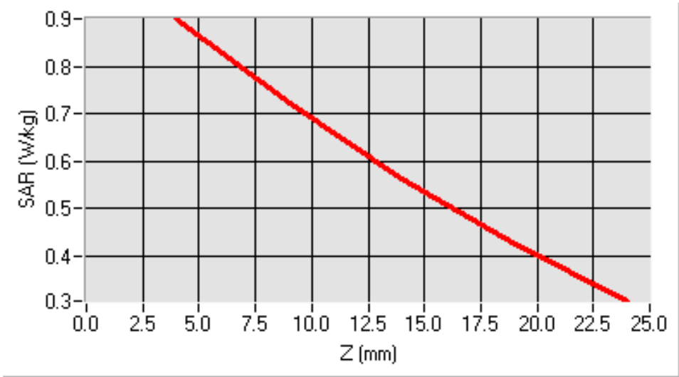
SAR, Z Axis Scan (X = -10, Y = -2)
