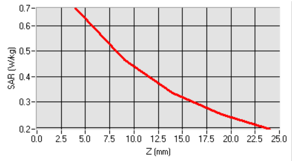
SAR, Z Axis Scan (X = -21, Y = -7)
