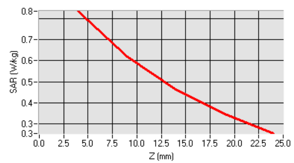
SAR, Z Axis Scan (X = -23, Y = -10)
