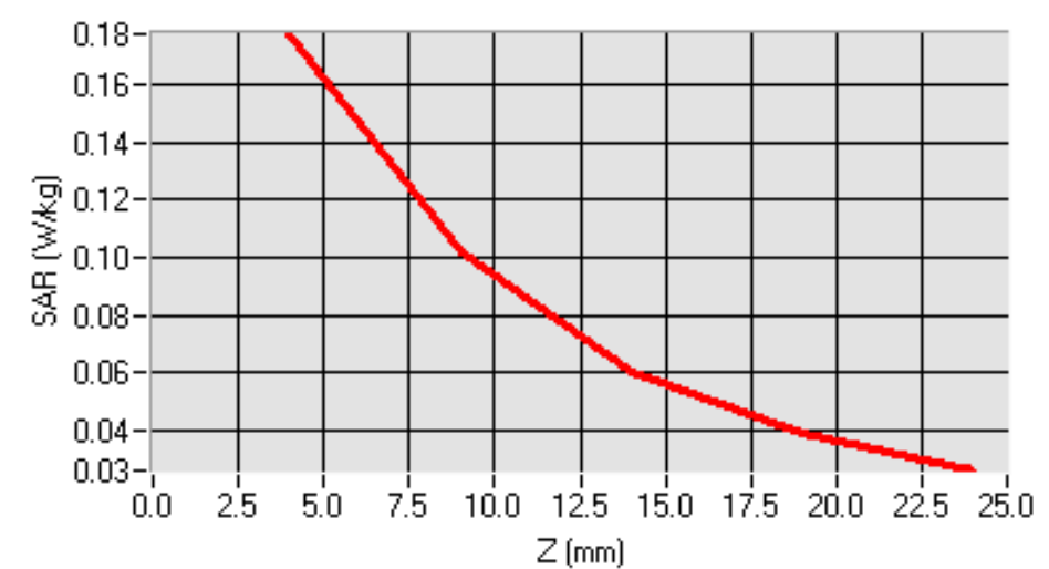
SAR, Z Axis Scan (X = -6, Y = -6)
