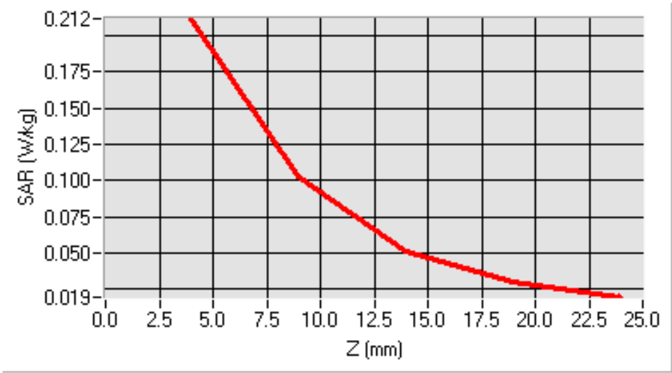
SAR, Z Axis Scan (X = -17, Y = 2)
