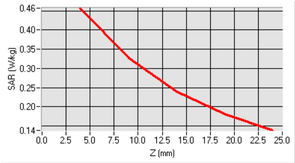
SAR, Z Axis Scan (X = 0, Y = -23)
