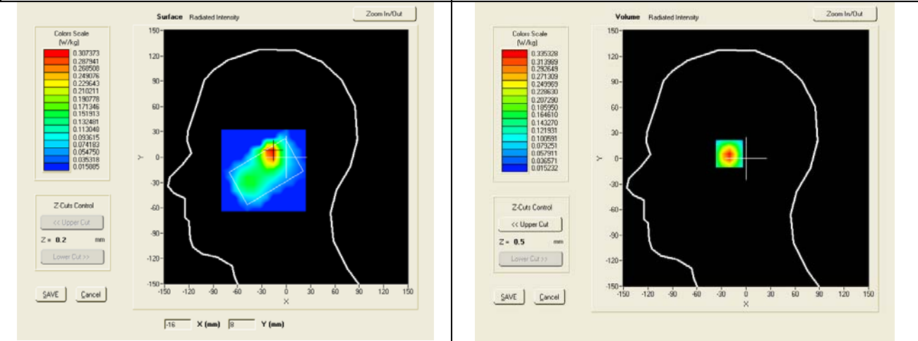
SAR, Z Axis Scan (X = -18, Y = 6)
