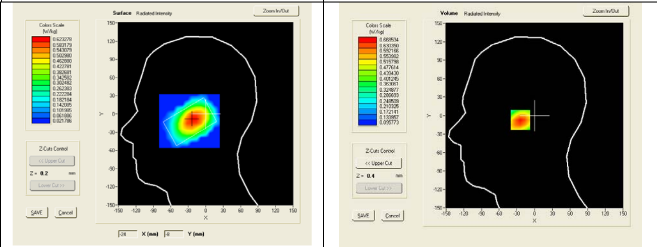
SAR, Z Axis Scan (X = -21, Y = -7)
