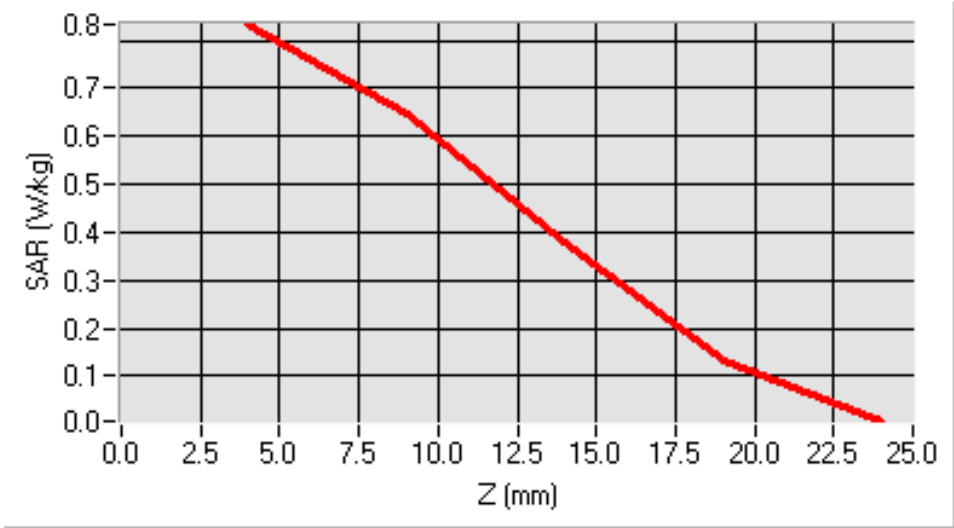
SAR, Z Axis Scan (X = -24, Y = -14)
