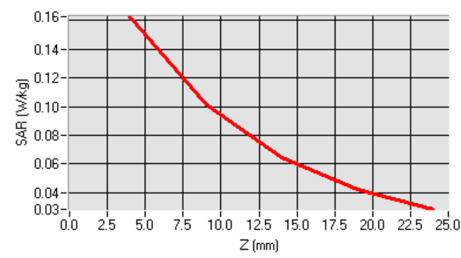
SAR, Z Axis Scan (X = -8, Y = -7)
