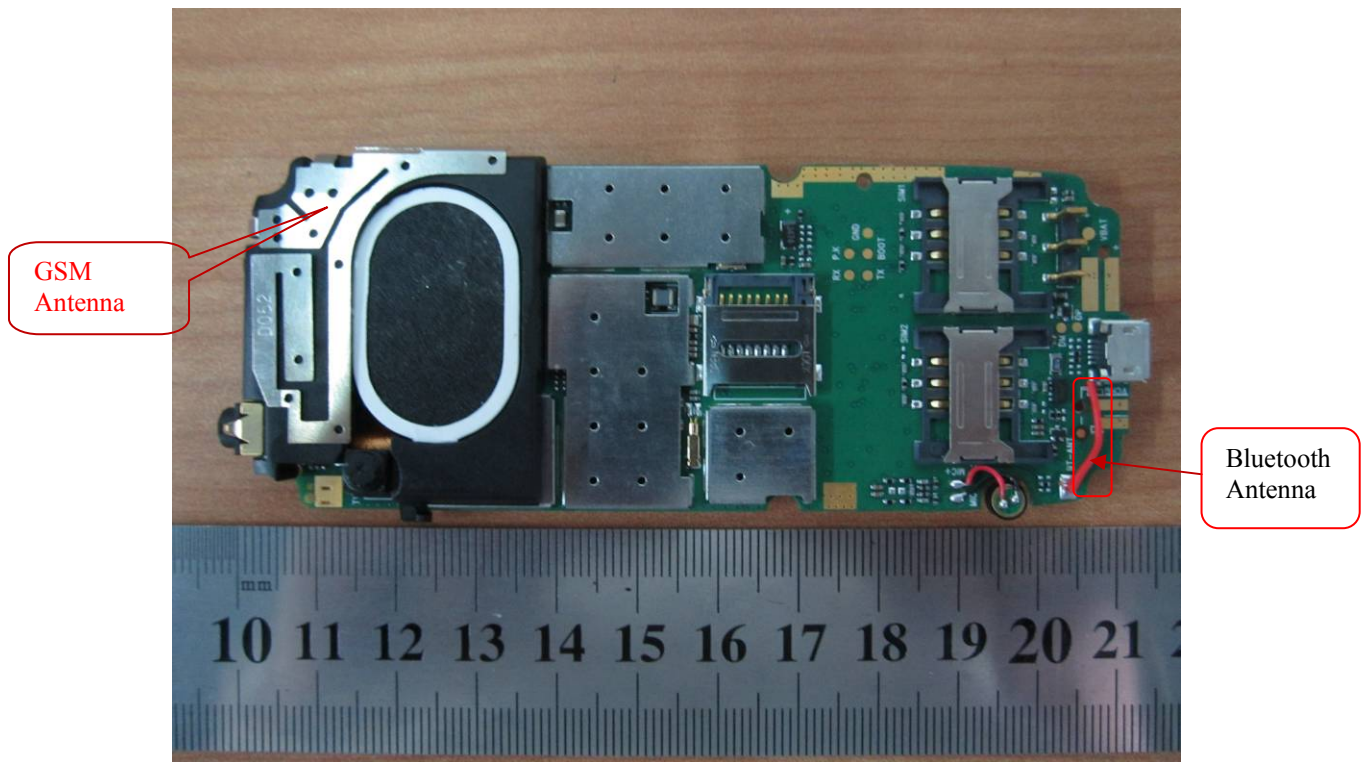
PCB Board view
