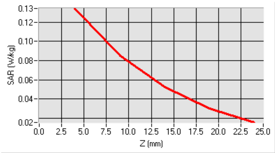
SAR, Z Axis Scan (X = 0, Y = -30)
