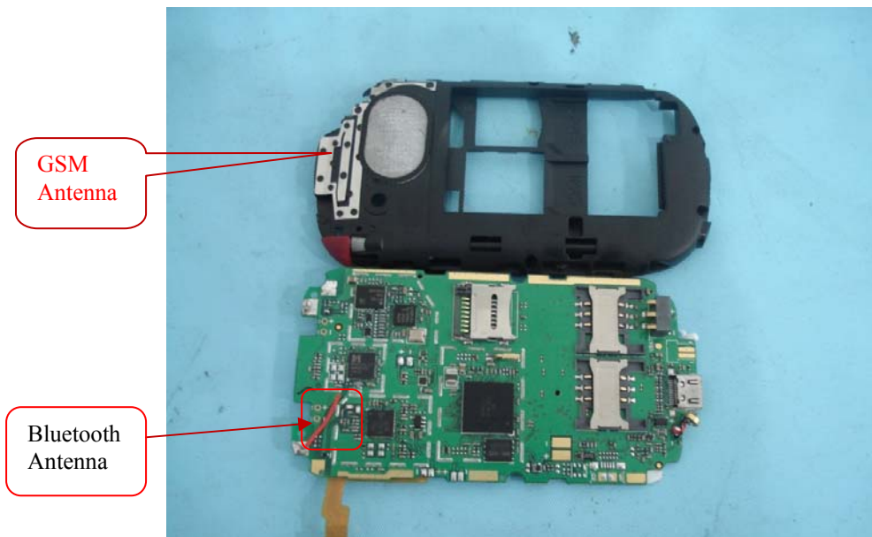
PCB Board view1
