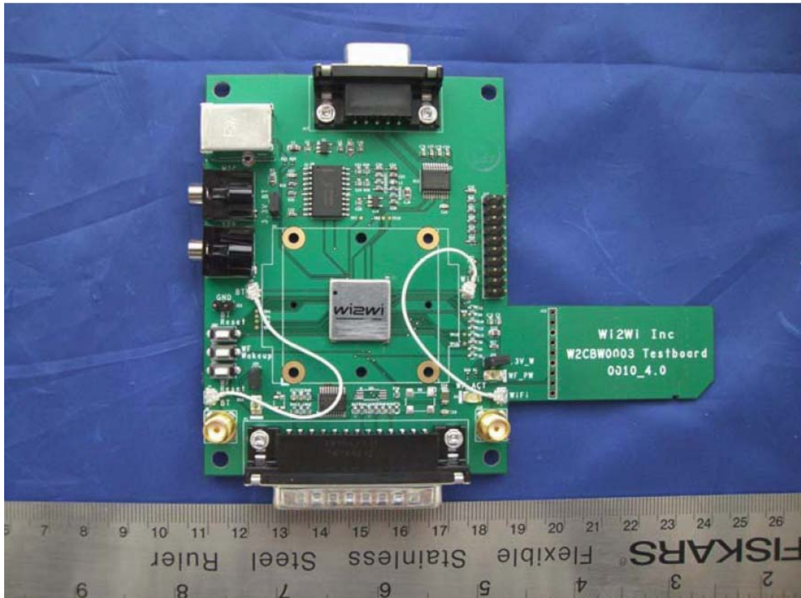
EUT with Test Board
