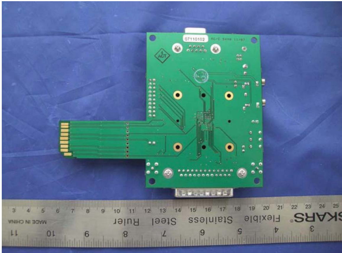
Test Board Solder Side View
