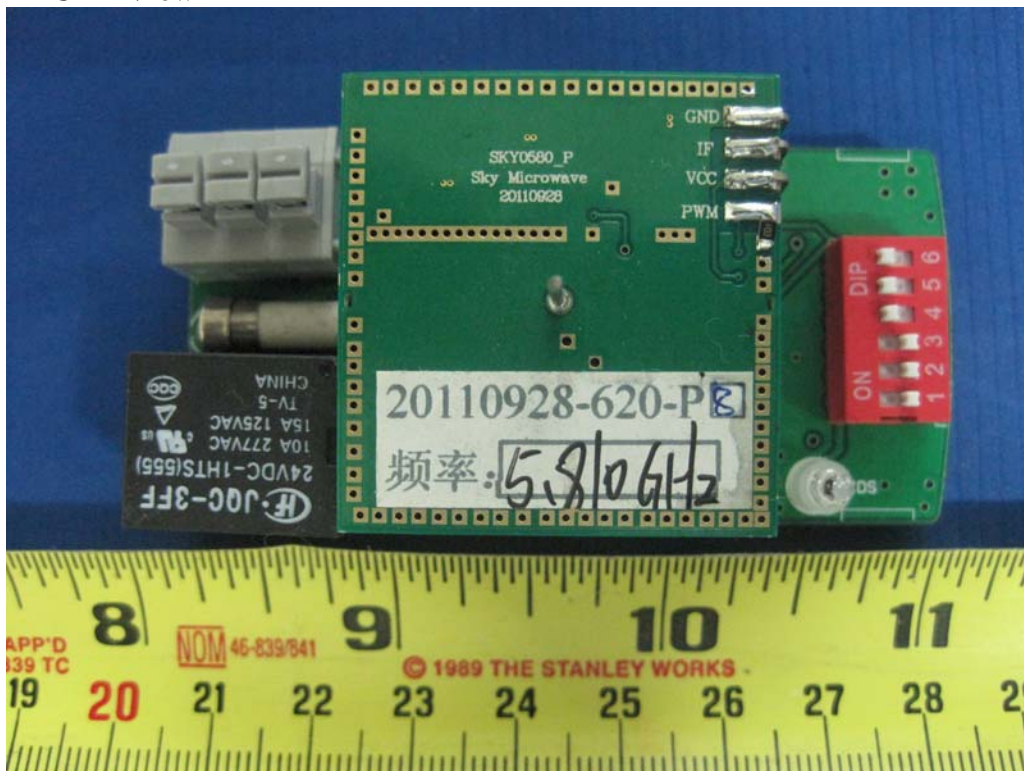
Main PCBA View
