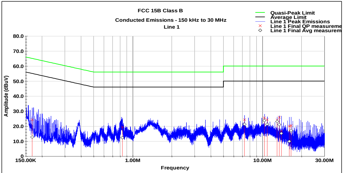
Line 1 Conducted Emissions Plot
