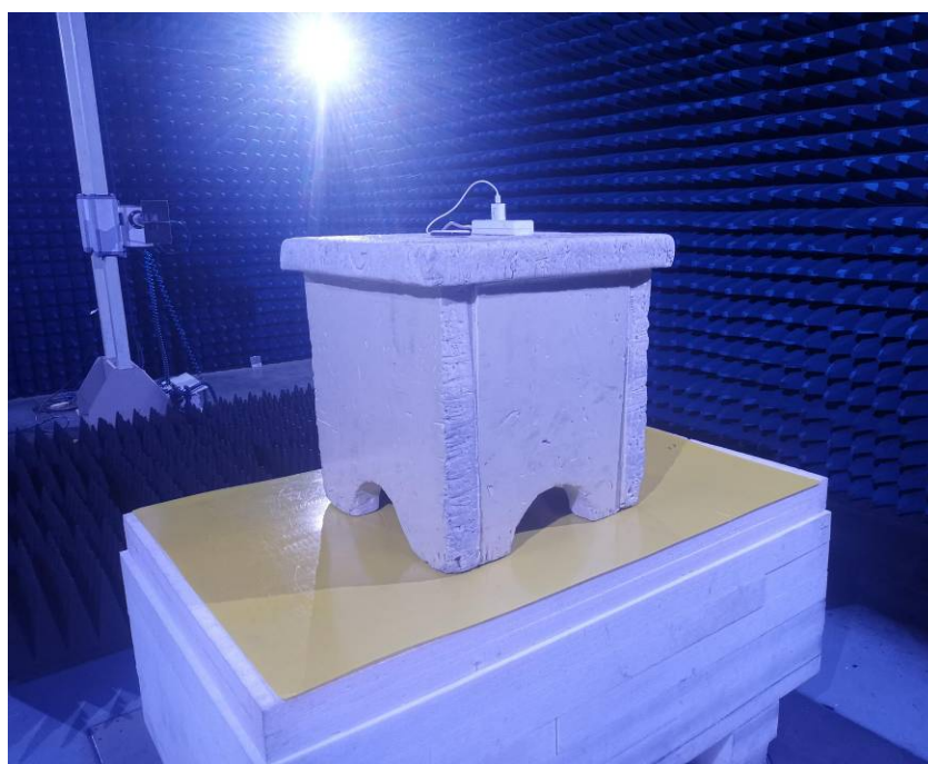
Photo of Radiated Emission Measurement (Above 1G)
