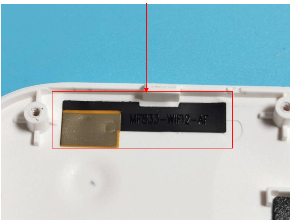
Wi-Fi ANT2
