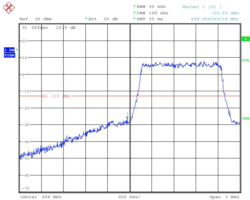
Band 12_1.4 MHz_Low_QPSK_RB6#0
