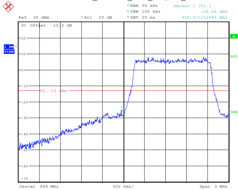
Band 12_1.4 MHz_Low_16QAM_RB6#0
