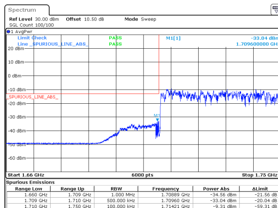
n66_40MHz_15kHz_1730MHz_DFT-s-OFDM QPSK_RB216@0
