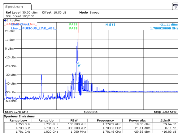
n66_30MHz_15kHz_1765MHz_DFT-s-OFDM QPSK_RB1@159
