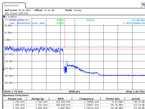
n66_30MHz_15kHz_1765MHz_DFT-s-OFDM QPSK_RB160@0
