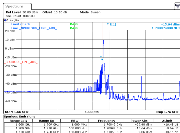
n66_40MHz_15kHz_1730MHz_DFT-s-OFDM QPSK_RB1@0
