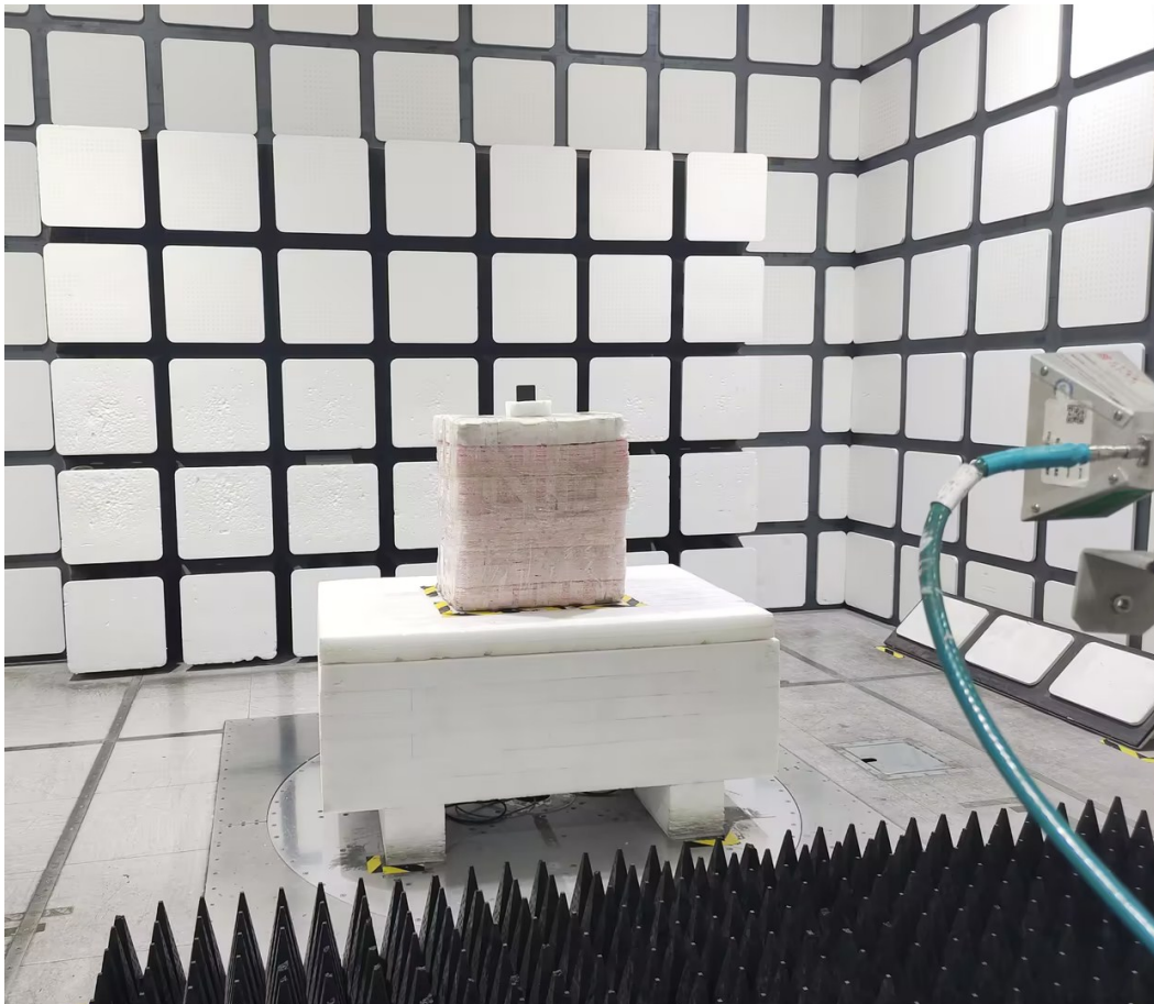
Radiated Emissions View (18-25 GHz)
