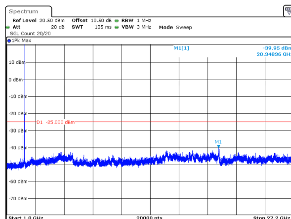
10MHz_High_QPSK_1@0(1GHz~27.2GHz)
