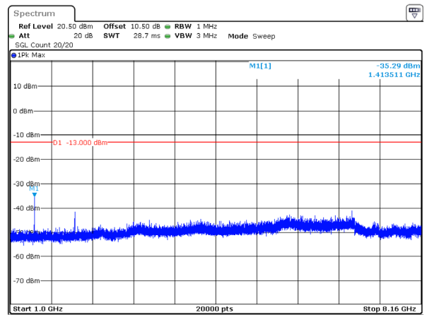
10MHz_High_QPSK_1@0(1GHz~8.16GHz)
