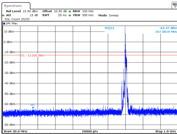
10MHz_High_QPSK_1@0(30MHz~1GHz)
