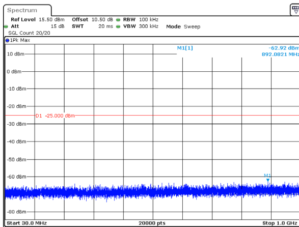
20MHz_Low_QPSK_1@0(30MHz~1GHz)
