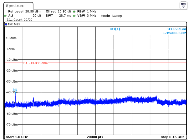
10MHz_Middle_QPSK_50@0(1GHz~8.16GHz)
