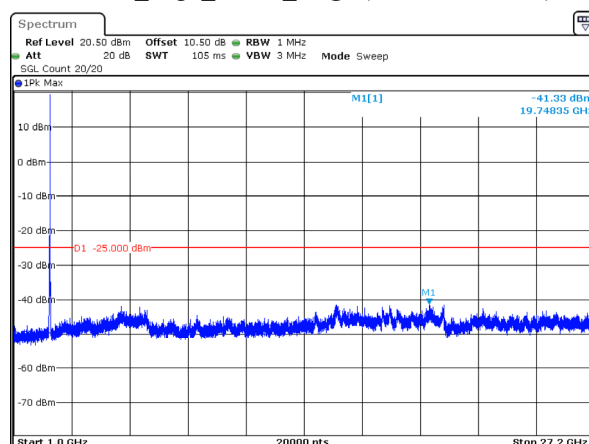
10MHz_High_QPSK_50@0(1GHz~27.2GHz)
