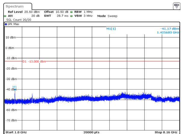
10MHz_High_QPSK_50@0(1GHz~8.16GHz)
