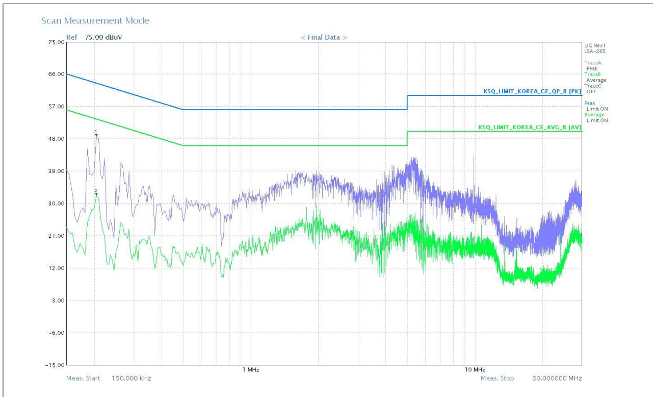
Neutral – PE(Peak and Average detector used)
