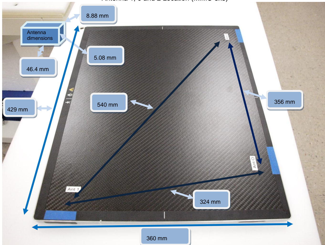
Antenna 1, 0 and 2 Location (MIMO 3x3)
