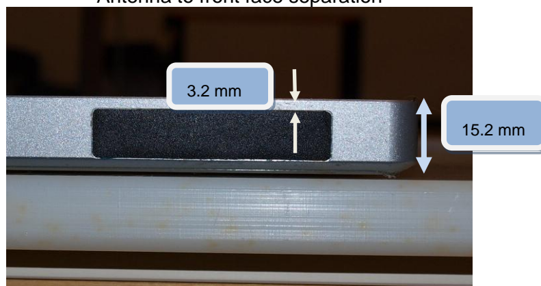
Antenna to front face separation
