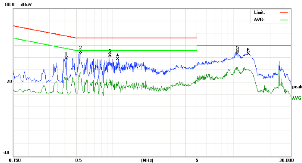
LINE CONDUCTED EMISSION – L
