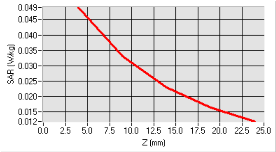
SAR, Z Axis Scan (X = 17, Y = -32)
