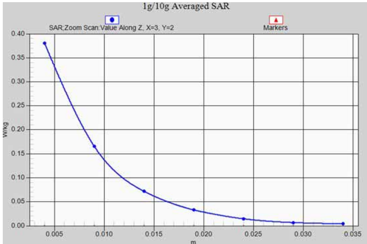
WiFi 802.11b RIGHT/CKEEK-Low _ z-axis scan
