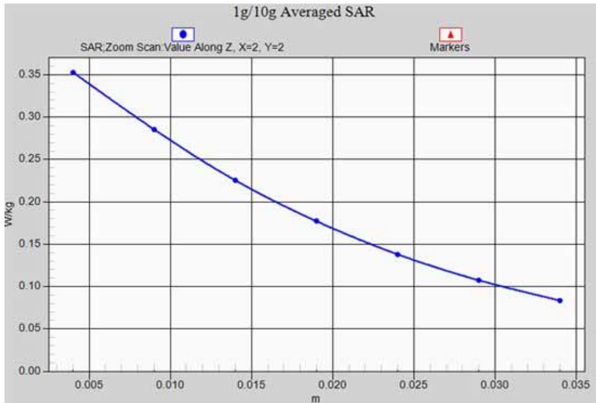
WCDMA Band V- LEFT/CHEEK-Mid _ z-axis scan
