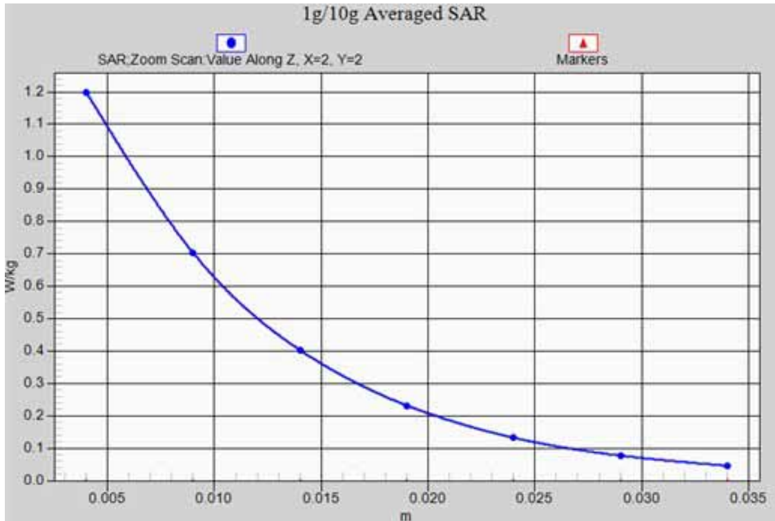
WCDMA Band II Body/Back side-High _ z-axis scan
