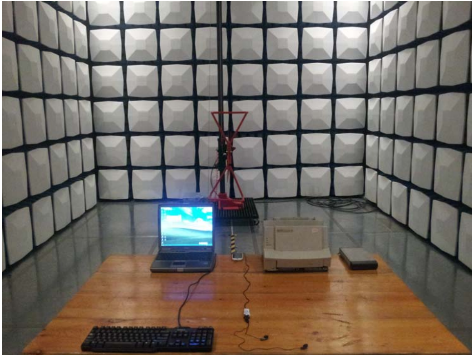
Radiated Emission (Downloading) - Rear View
