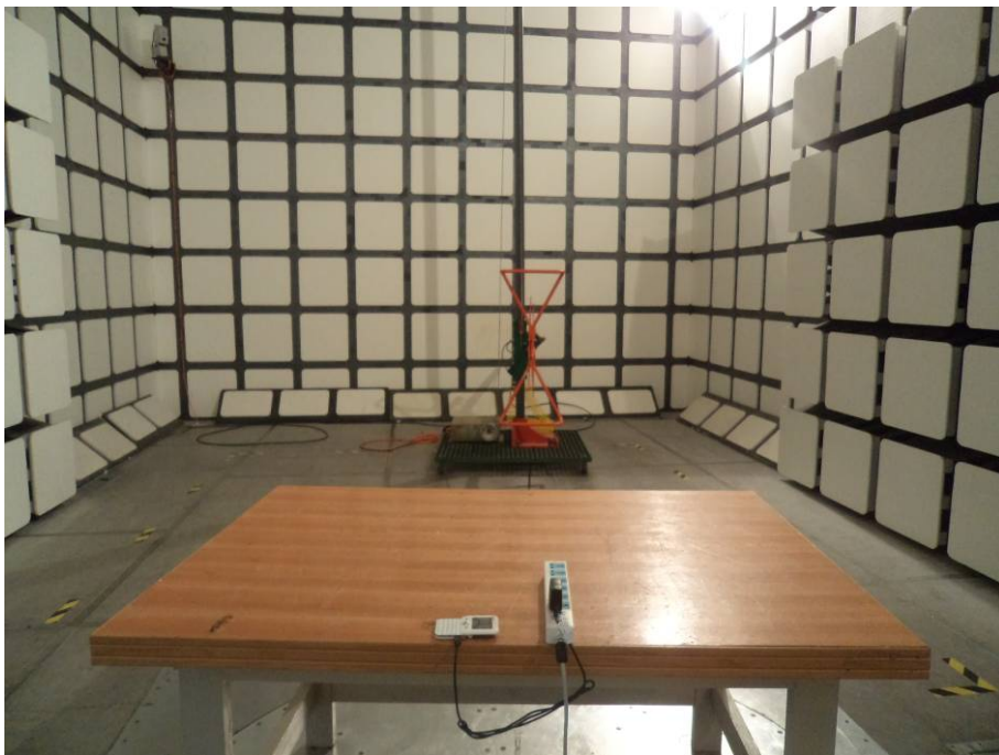
Radiated Emissions - Rear View (Charging & Media Playing)
