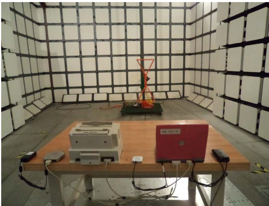
Spurious Radiated Emissions - Rear View (Downloading mode)
