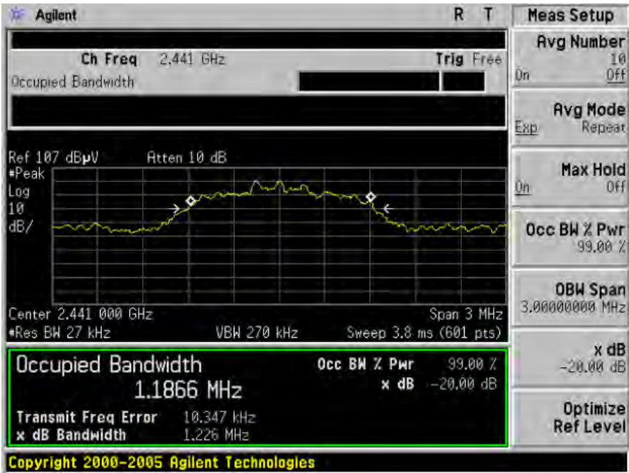
TEST PLOT OF BANDWIDTH FOR MIDDLE CHANNEL
