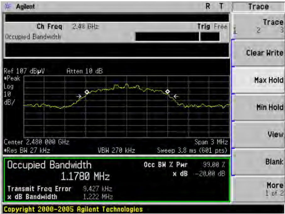
TEST PLOT OF BANDWIDTH FOR HIGH CHANNEL
