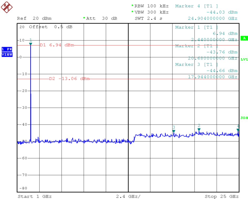
Mid Channel 1GHz to 25GHz @ GFSK Mode
