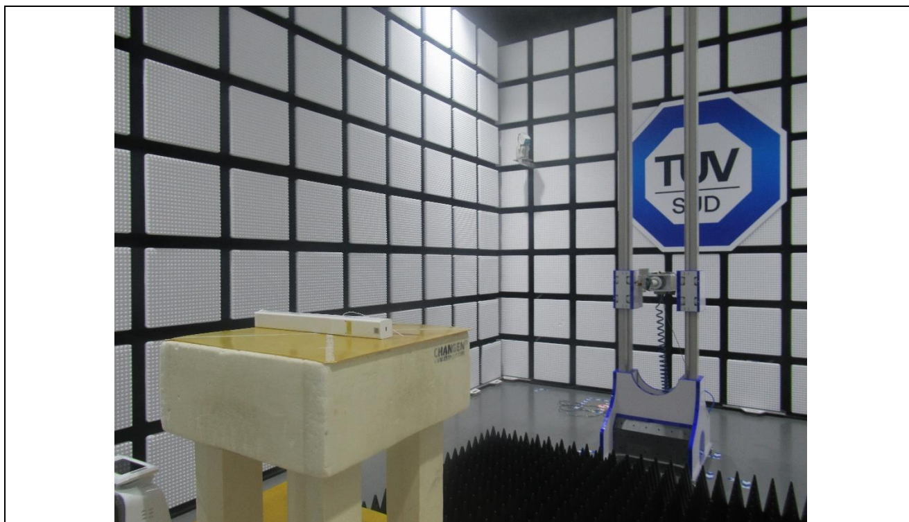
Radiated Emission test (18000-26500MHz)
