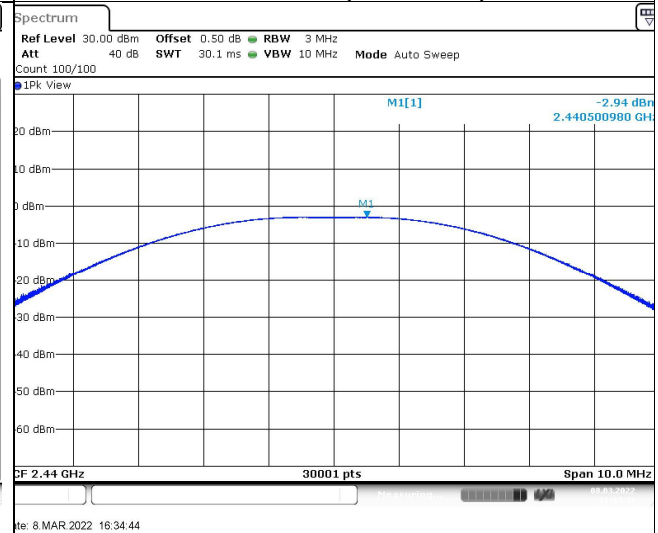
Channel 19 (2440MHz)
