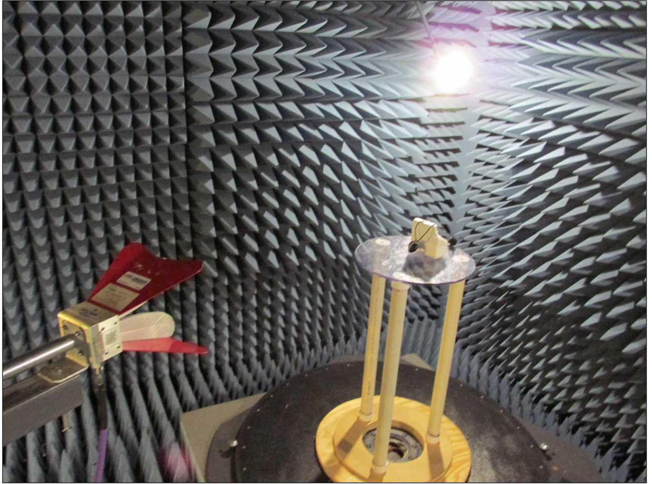
Photograph 2. Radiated Emissions, Test Setup, Above 1 GHz
