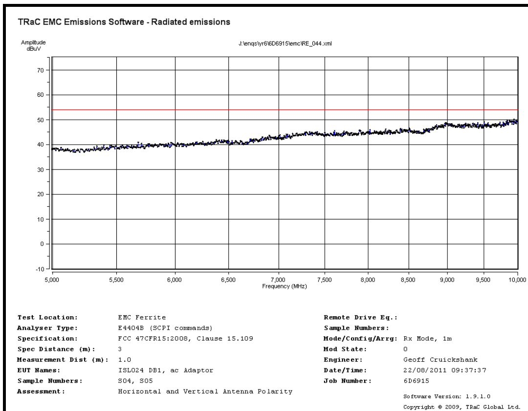
Radiated Spurious emissions 5 GHz to 10 GHz – Rx mode ac mains powered
