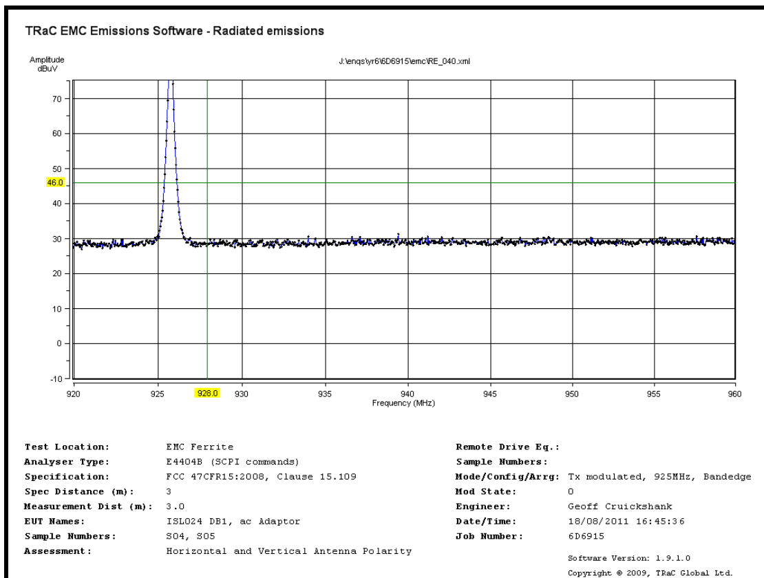
Upper Bandedge
