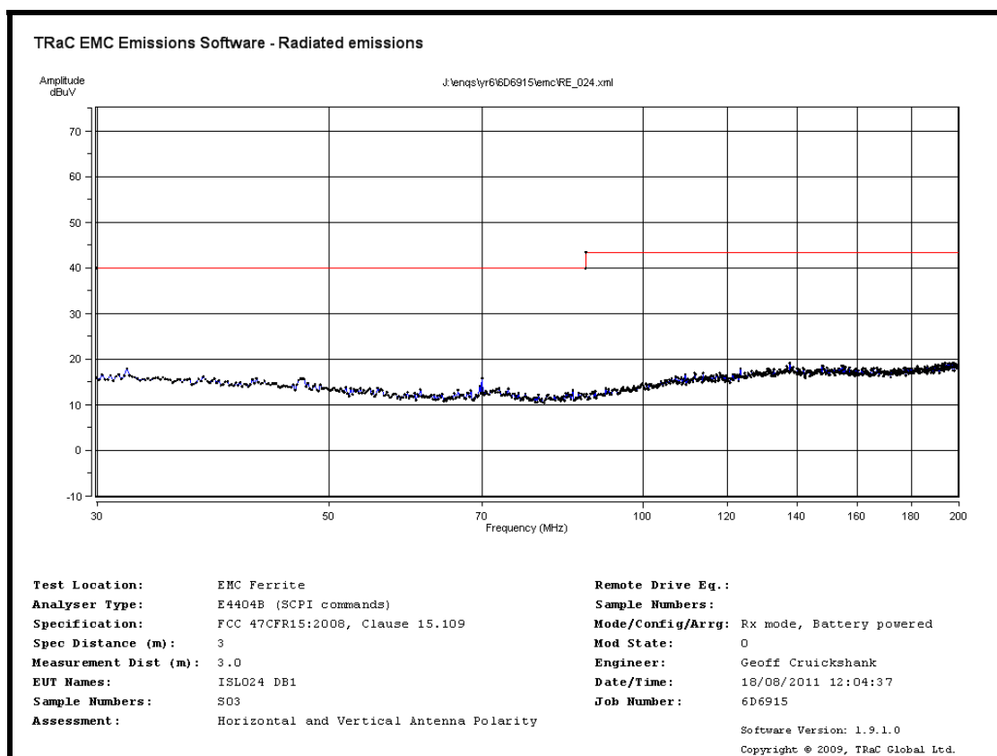
Radiated Spurious emissions 30 MHz to 200 MHz – Rx mode battery powered
