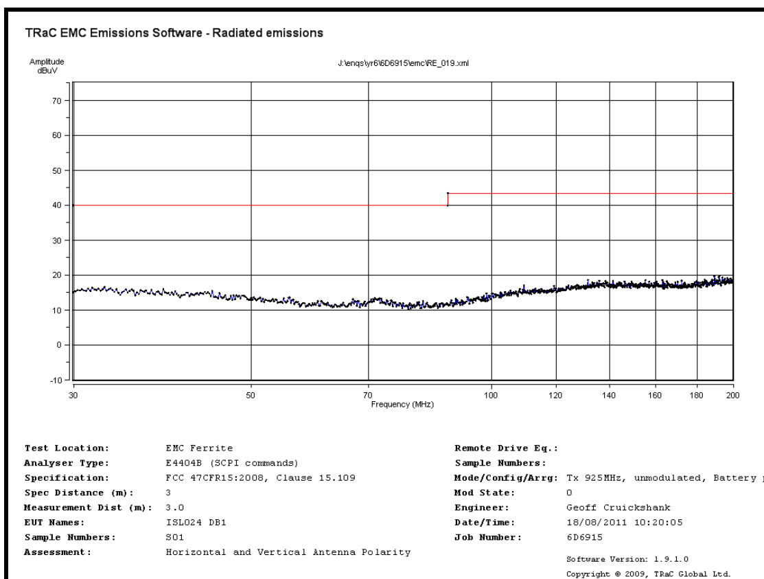
Radiated Spurious emissions 30 MHz to 200 MHz – Tx mode battery powered
