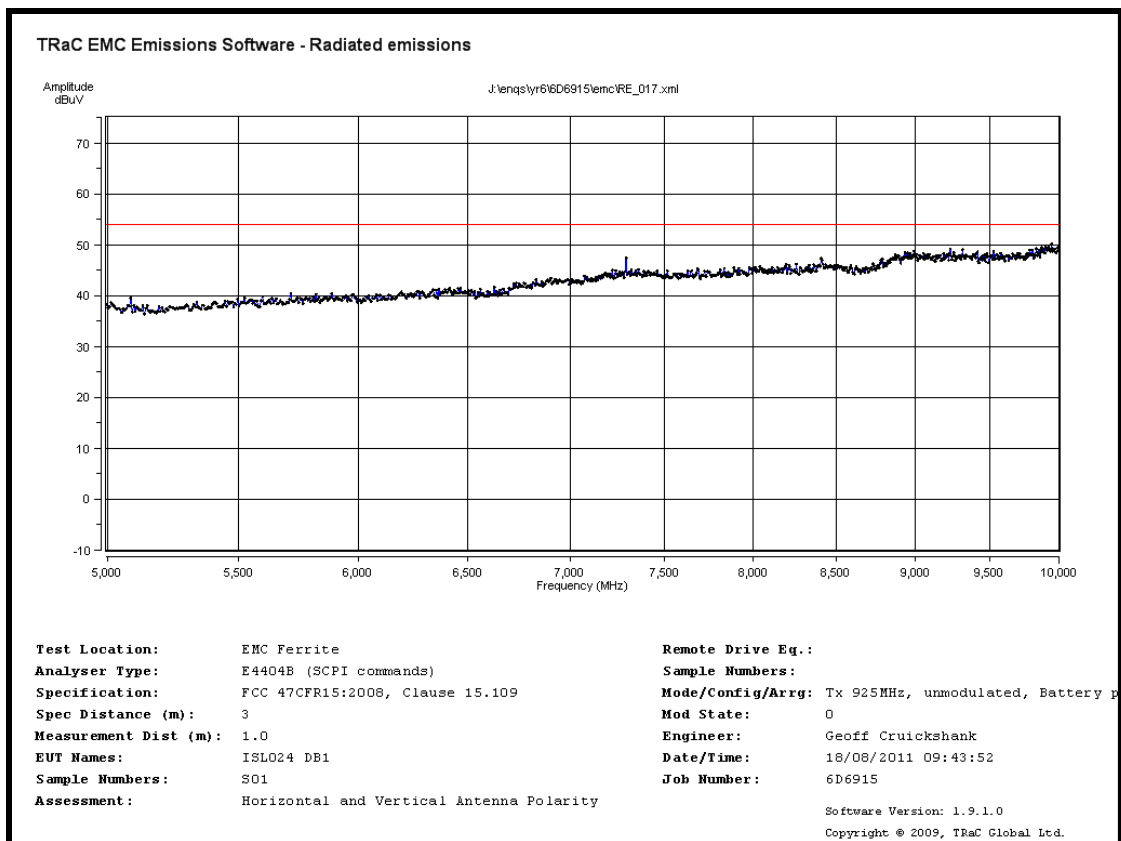
Radiated Spurious emissions 5 GHz to 10 GHz – Tx mode battery powered
