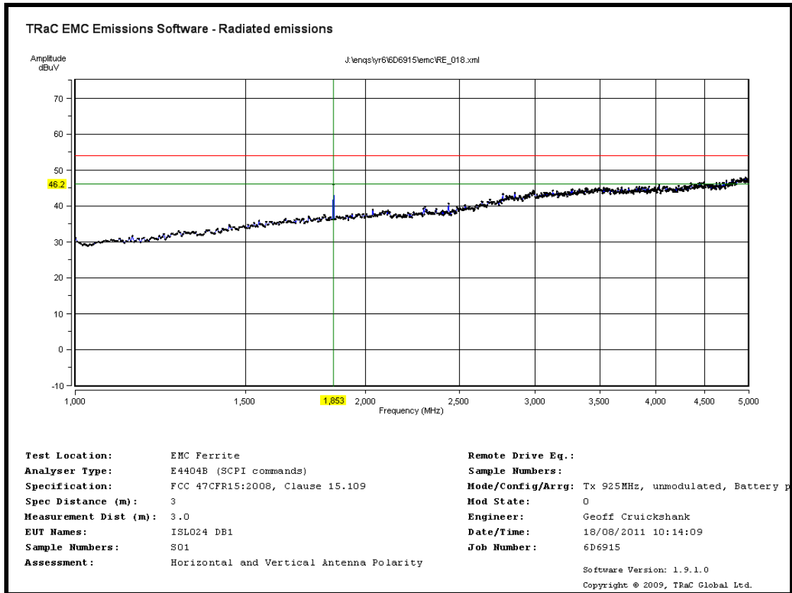
Radiated Spurious emissions 1 GHz to 5 GHz – Tx mode battery powered
