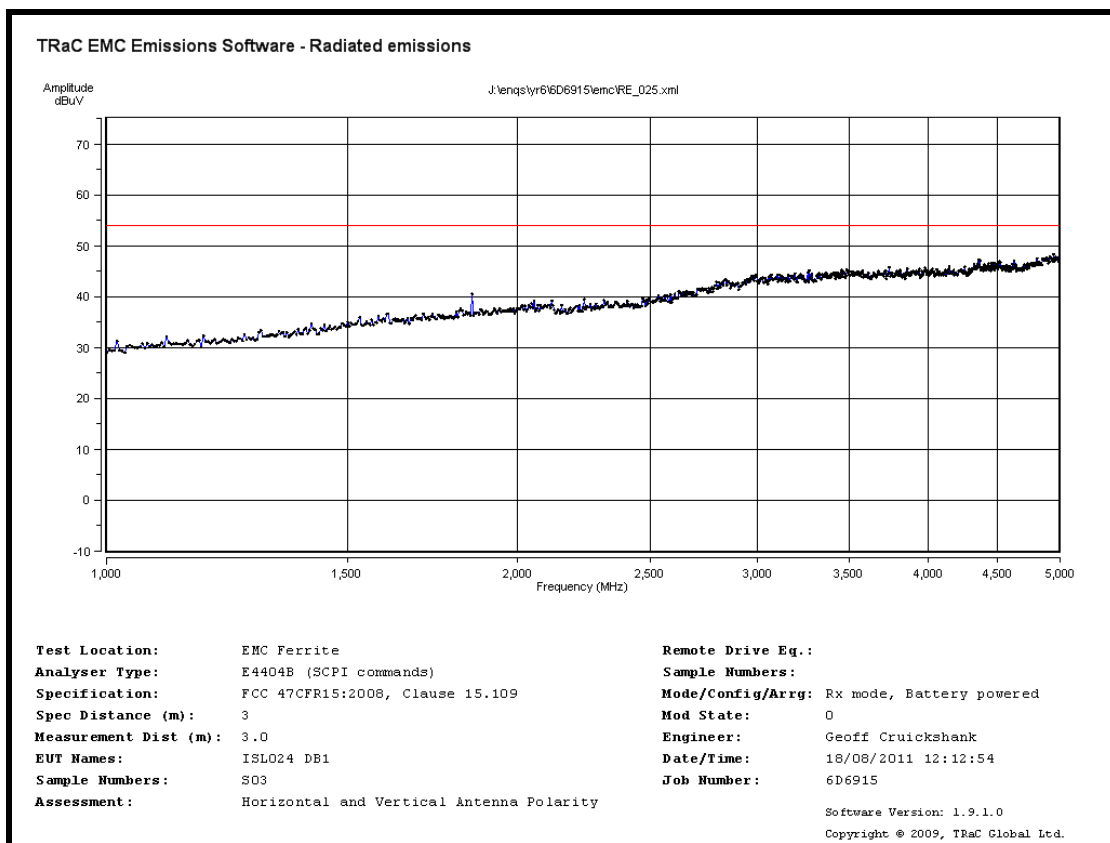
Radiated Spurious emissions 1 GHz to 5 GHz – Rx mode battery powered
