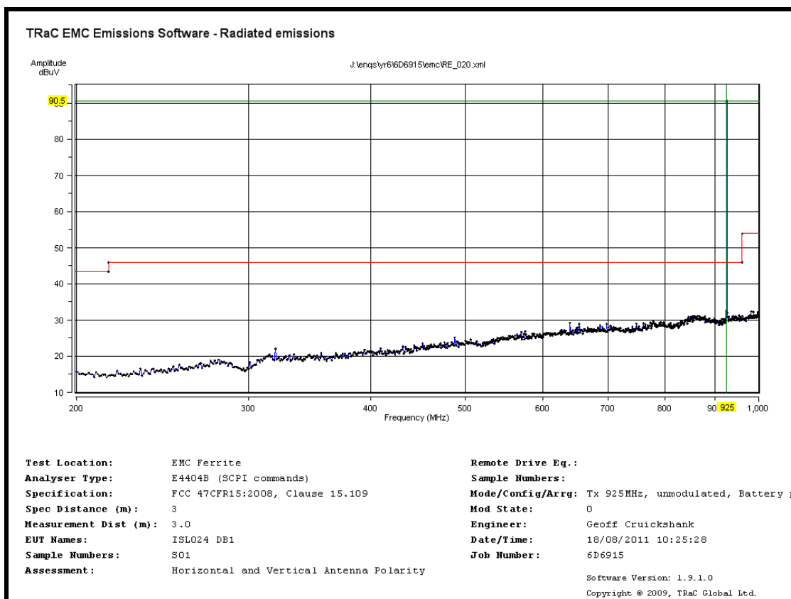
Radiated Spurious emissions 200 MHz to 1 GHz – Tx mode battery powered
