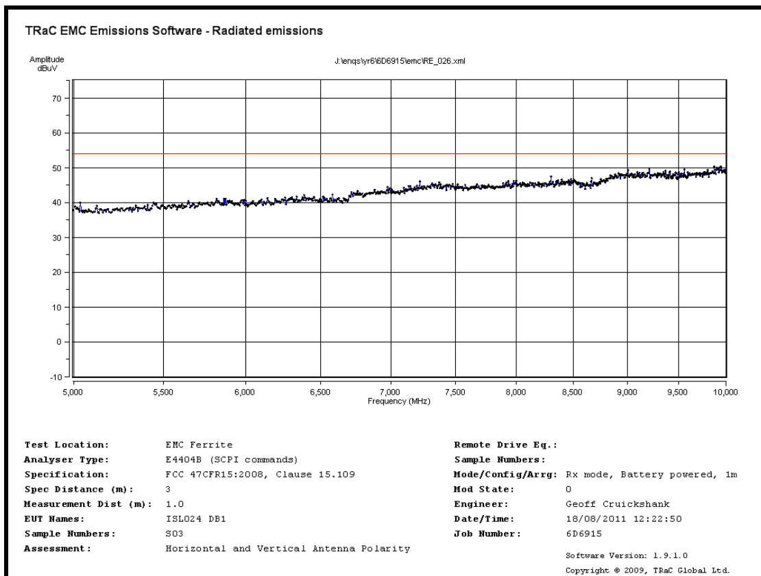
Radiated Spurious emissions 5 GHz to 10 GHz – Rx mode battery powered
