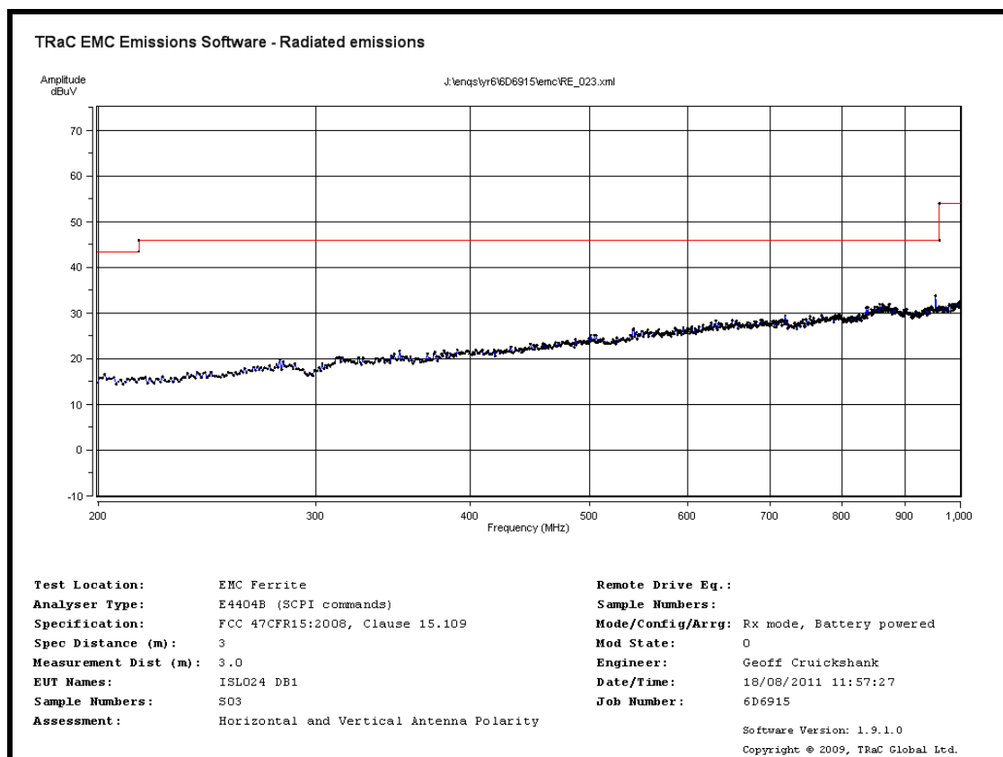
Radiated Spurious emissions 200 MHz to 1 GHz – Rx mode battery powered
