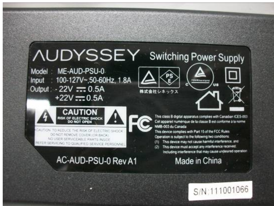
VIEW PHOTO OF AC Adapter
