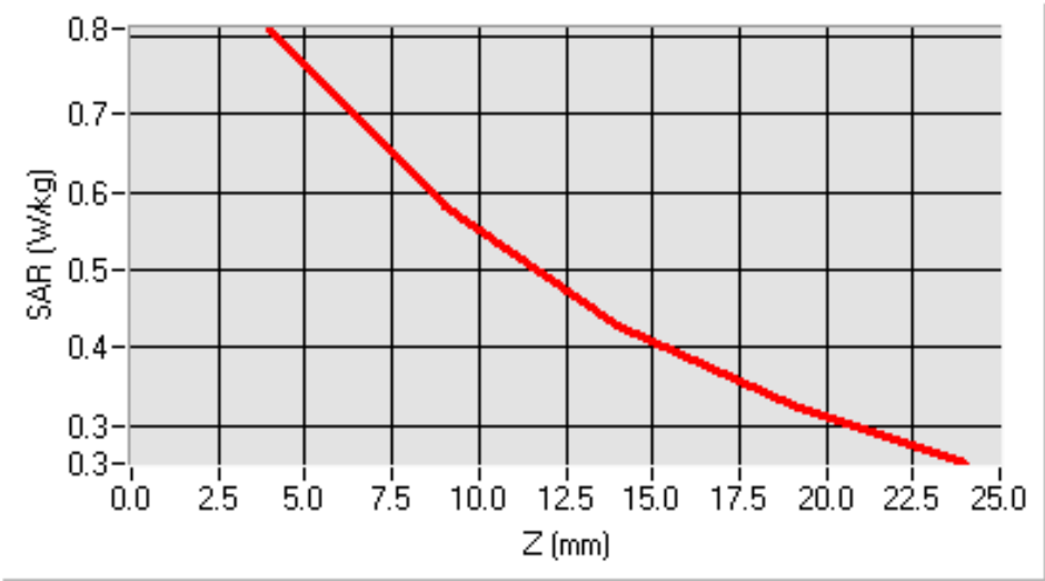
SAR, Z Axis Scan (X = -22, Y = -9)
