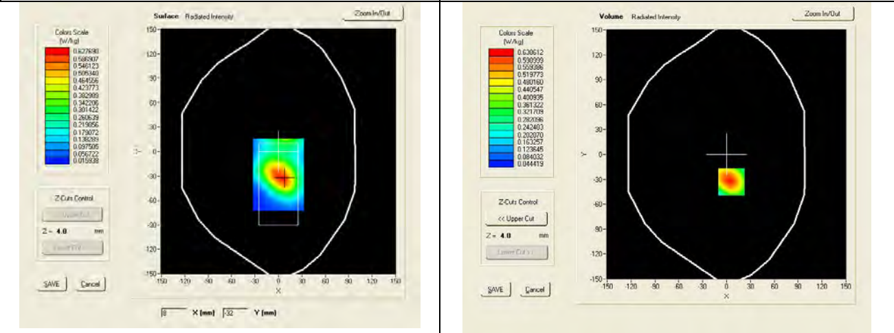
SAR, Z Axis Scan (X = 6, Y = -33)
