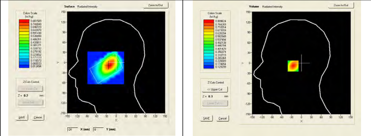
SAR, Z Axis Scan (X = -22, Y = -9)
