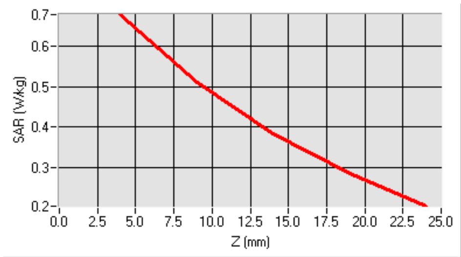
SAR, Z Axis Scan (X = -24, Y = -11)
