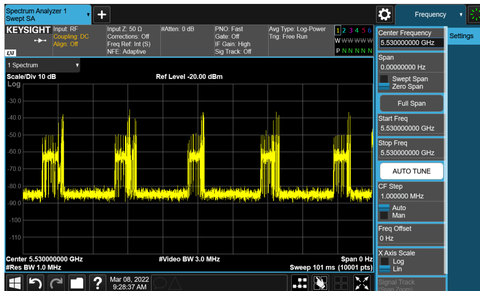
Channel Loading Plot - 802.11ac80-5530MHz
