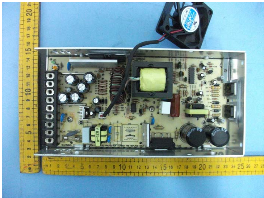
Figure 18 PCB-Front View
