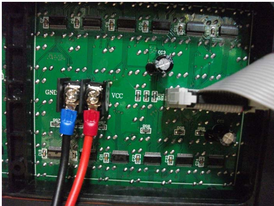
Figure 14 The EUT-Inside View
