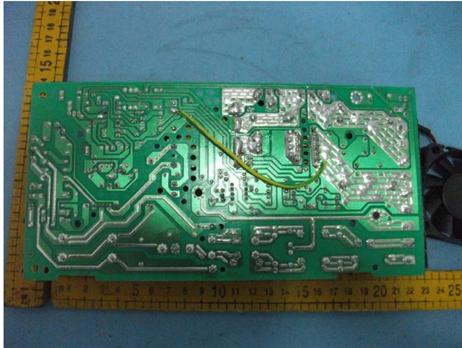
Figure 19 PCB-Back View
