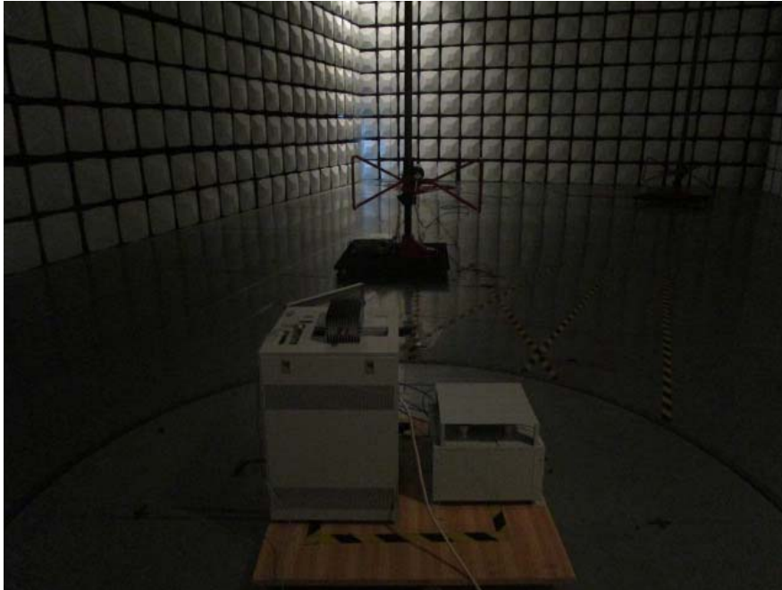
Transmitting Radiated Emissions Below 1 GHz– Rear View (AC Source With Combiner)
