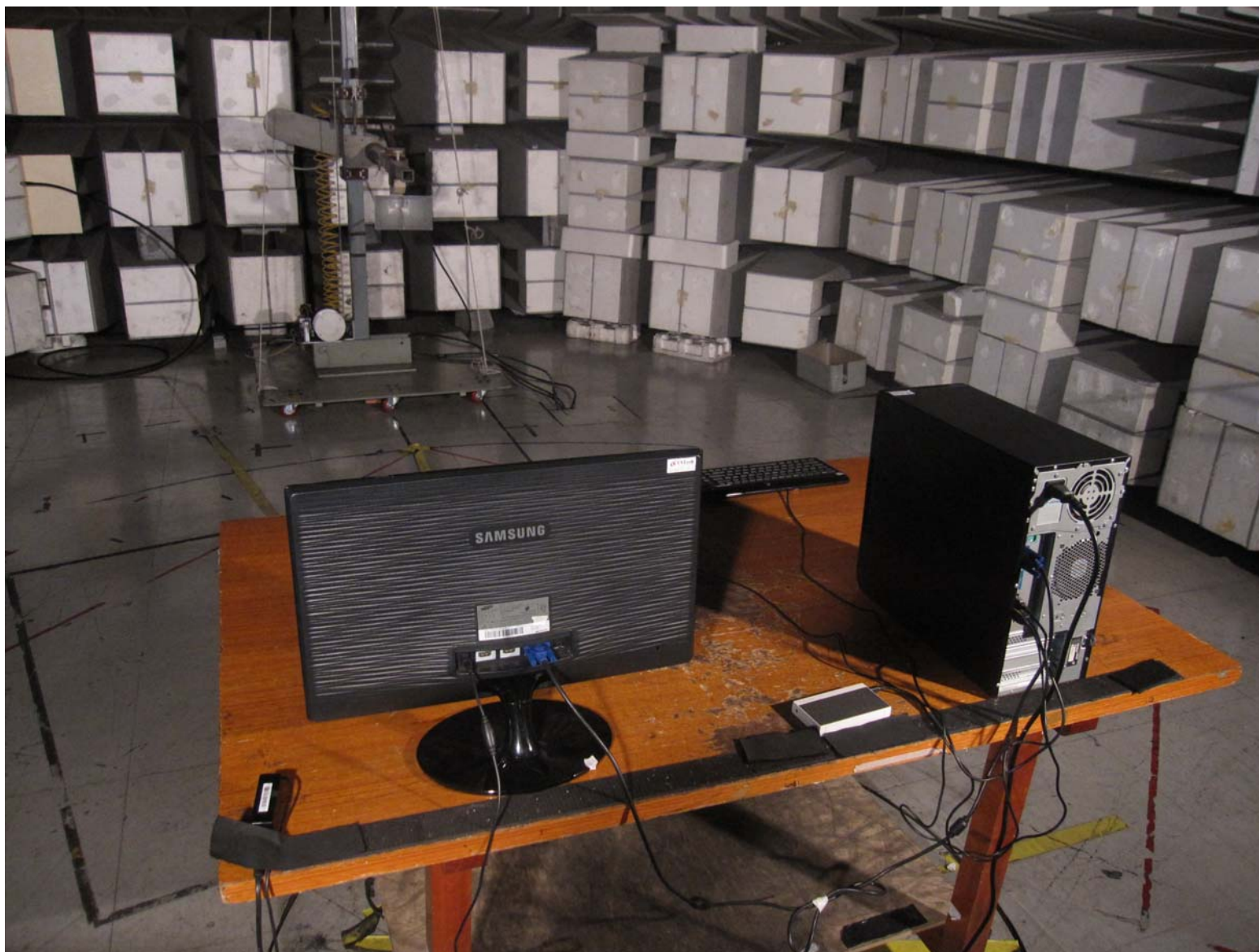
Radiated_1 GHz to 12.75 GHz_USB Charging status_Rear View
