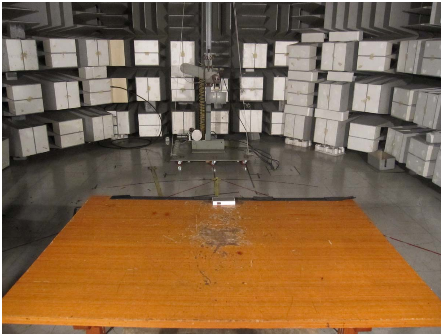
Radiated_1 GHz to 12.75 GHz_X axis Portable_Front View
