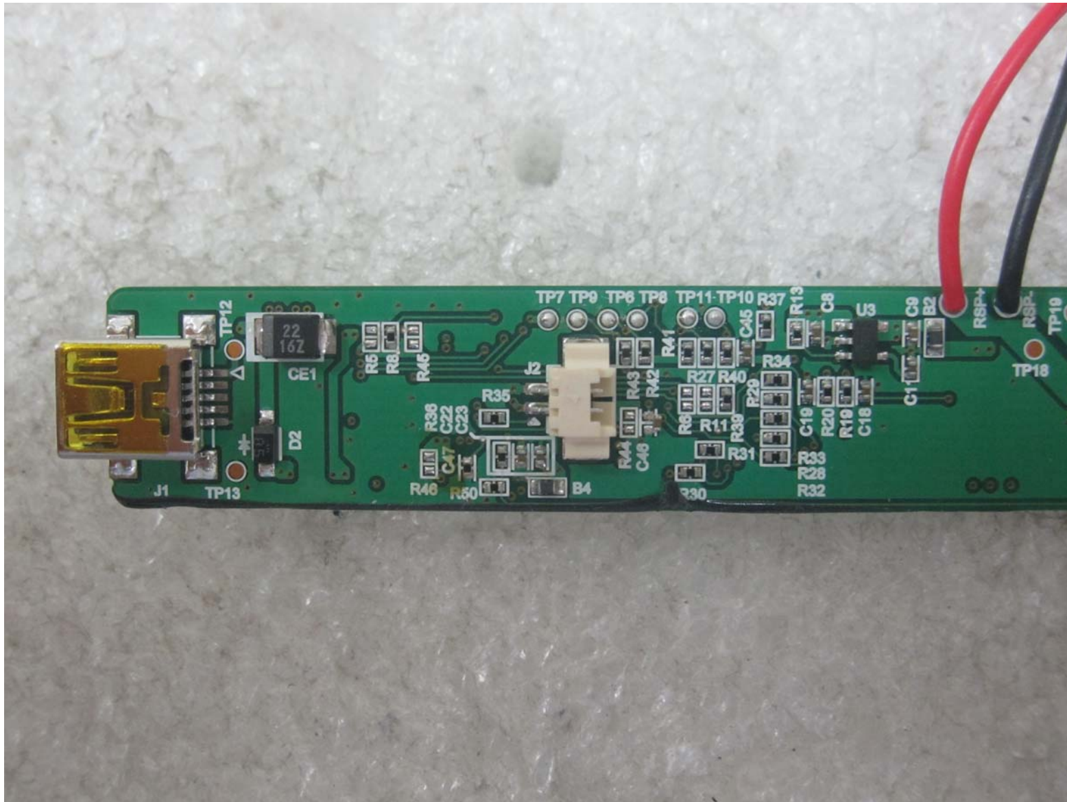
EXB100_Main Board Rear view-1
