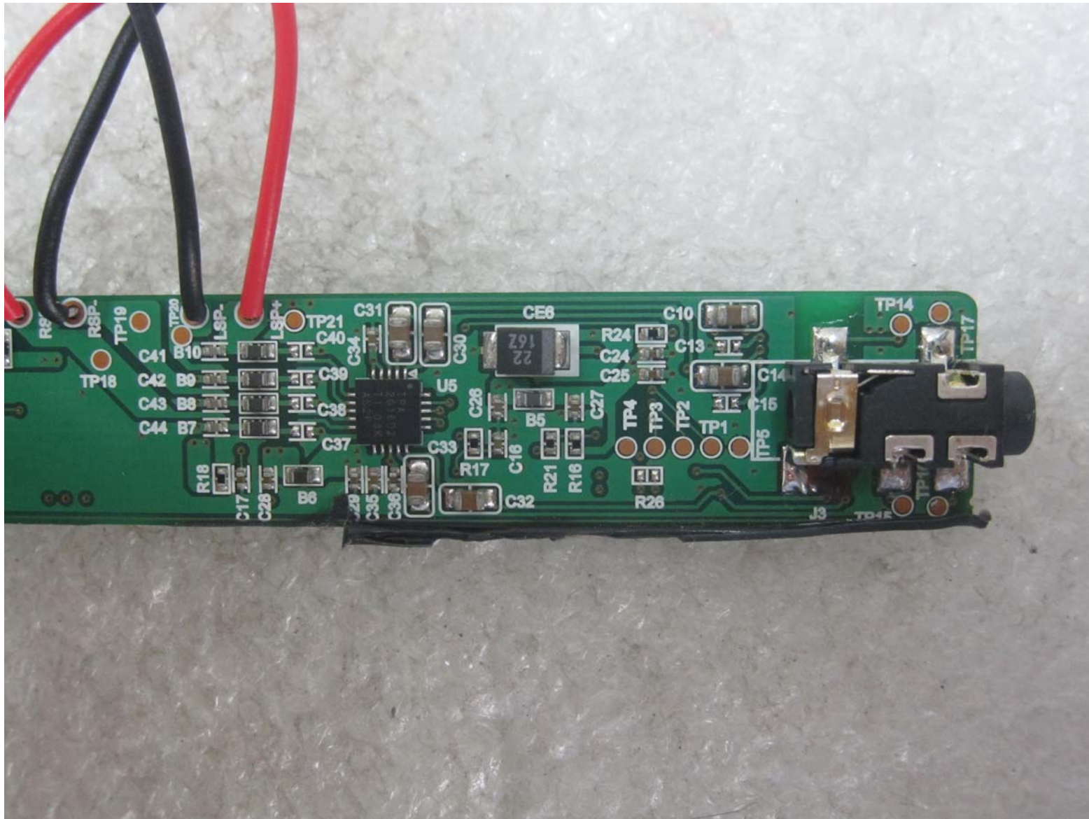
EXB100_Main Board Rear view-2
