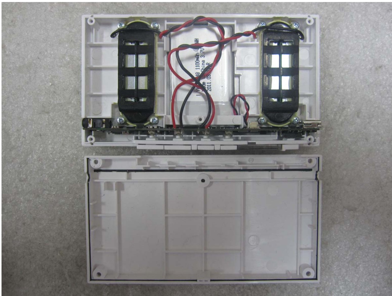
EXB100_Inside view
