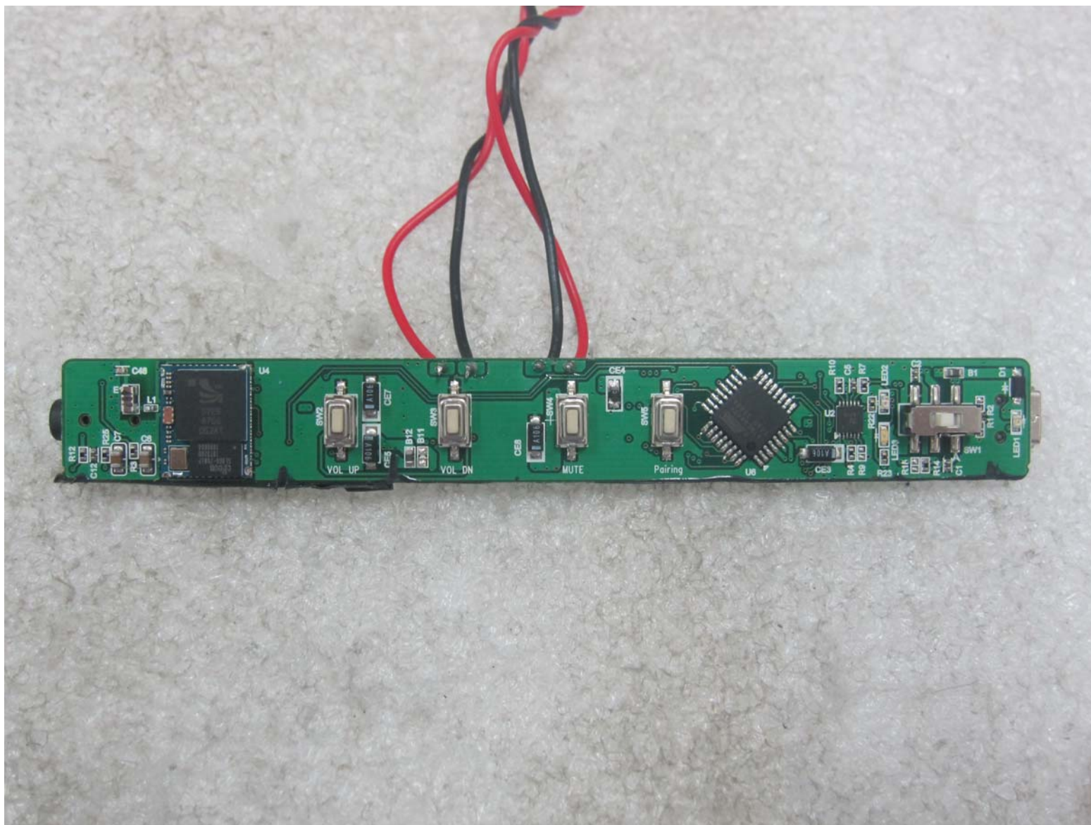
EXB100_Main Board Front view (RF Module Inside view)
