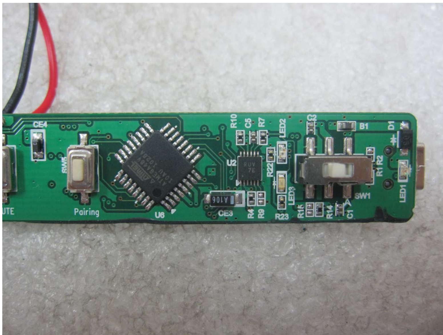
EXB100_Main Board Front view-2
