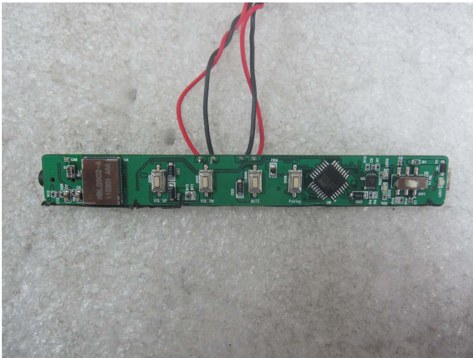
EXB100_Main Board Front view
