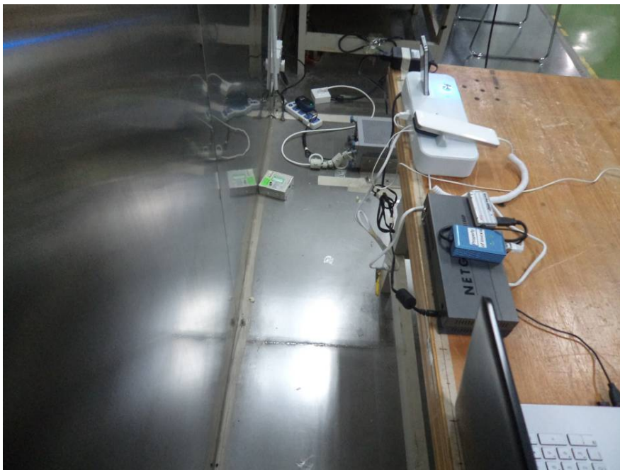
Conducted Disturbance - Side View (PoE power supply)
