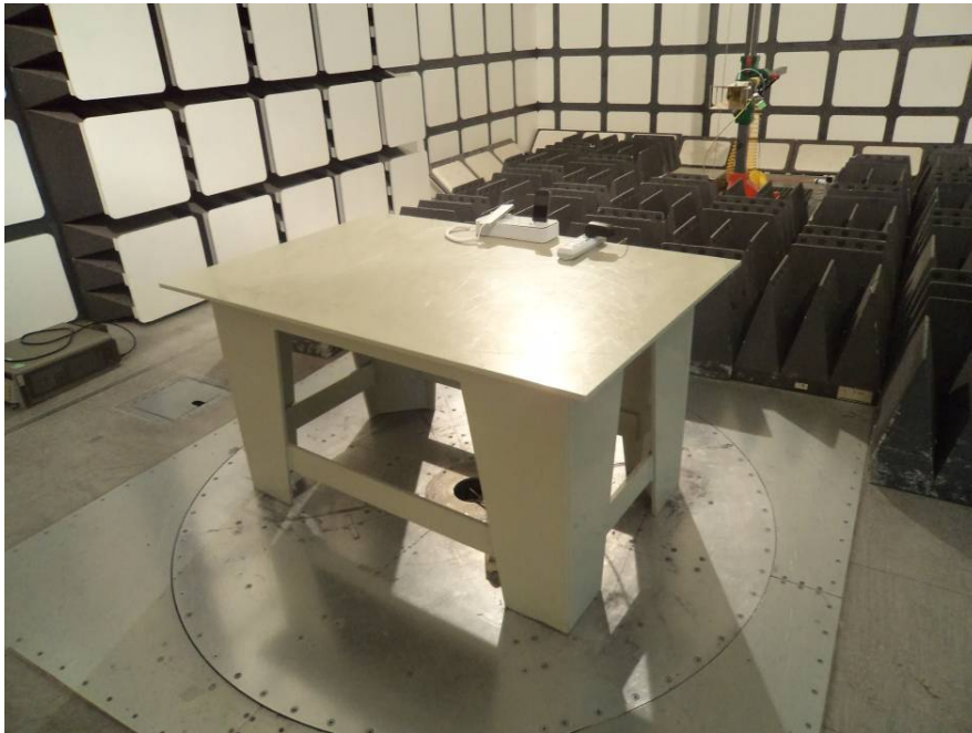
Above 1 GHz: Radiated Disturbance - Front View (Adapter power supply)
