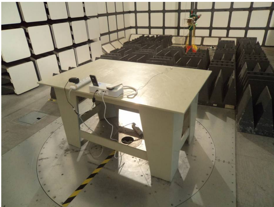
Above 1 GHz: Radiated Disturbance - Rear View (Adapter power supply)
