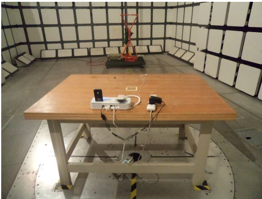
Below 1 GHz: Radiated Disturbance - Rear View (Adapter power supply)
