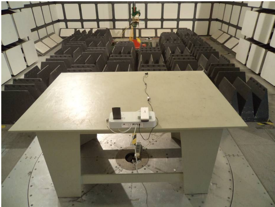
Above 1 GHz: Radiated Disturbance - Rear View (PoE power supply)
