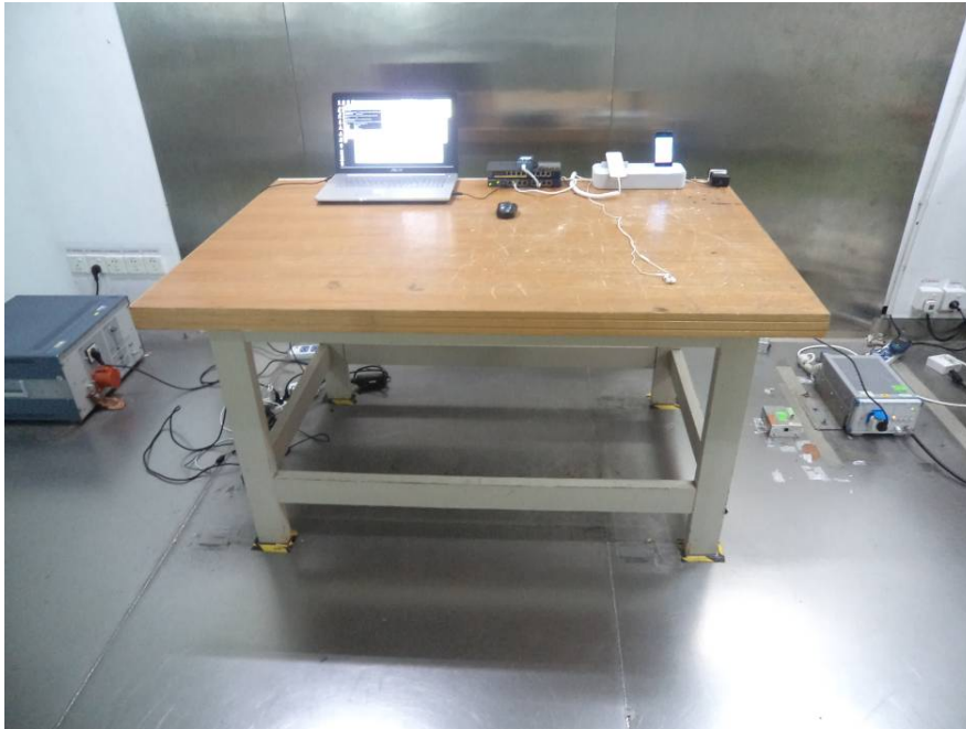
Conducted Disturbance - Front View (PoE power supply)
