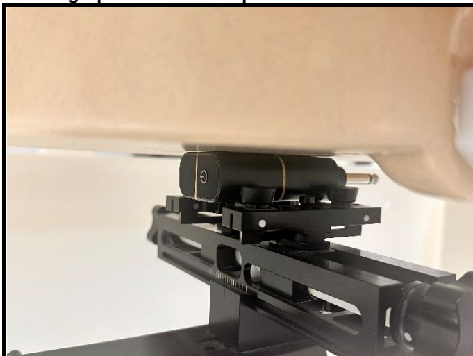
Front Face (EUT with 0 cm Gap)
