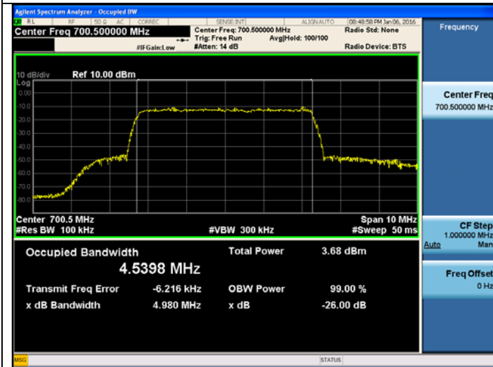
[700 Band AGC threshold Uplink Output LTE 5 MHz High]
