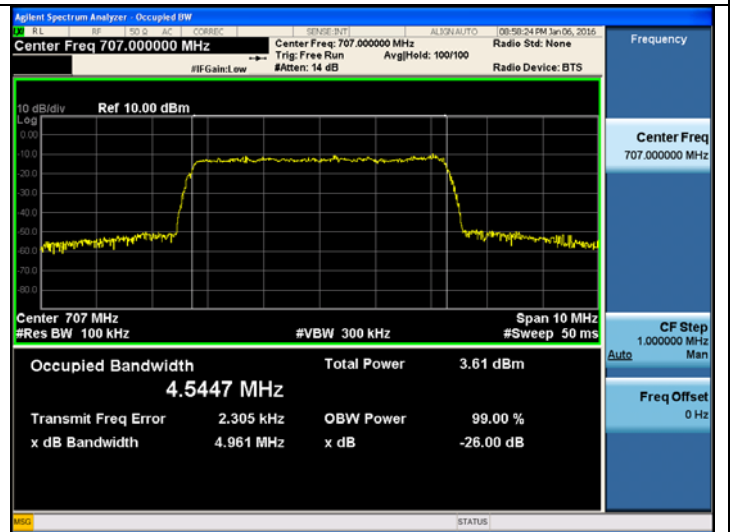
[700 Band AGC threshold Uplink Output LTE 5 MHz Mid]
