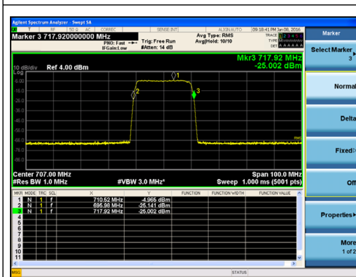
[700M Band Uplink 1]
