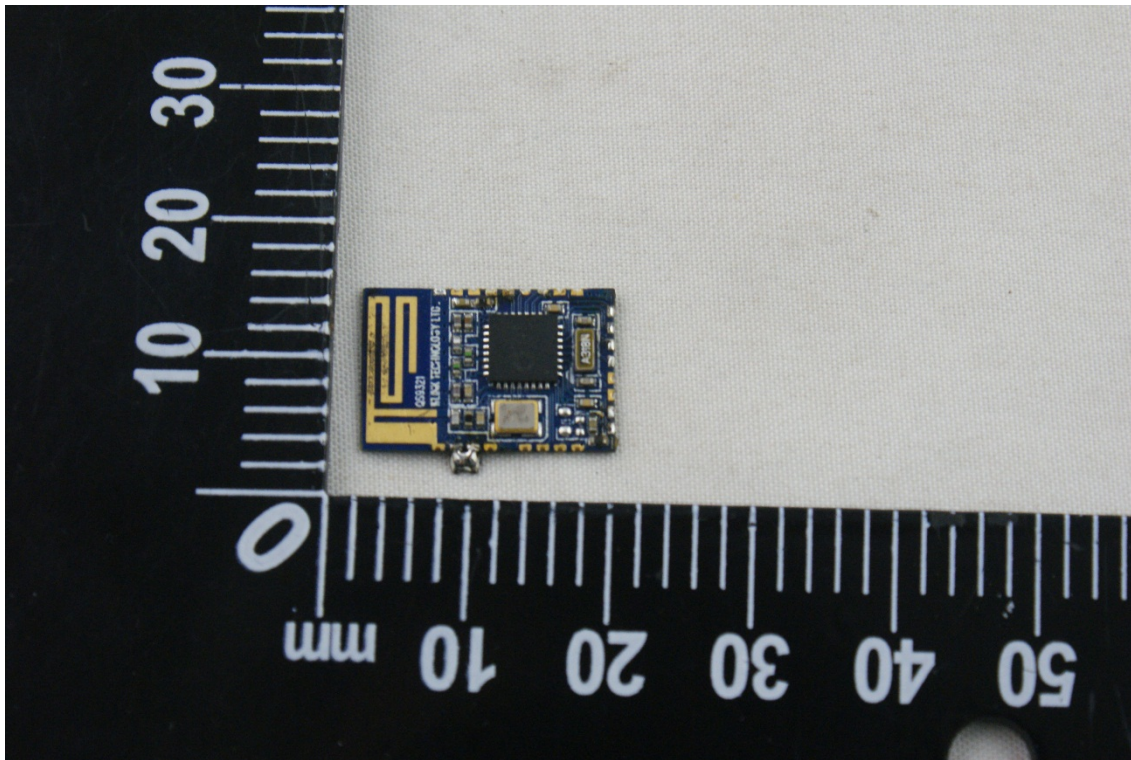
MODULE 2 TOP VIEW 6
