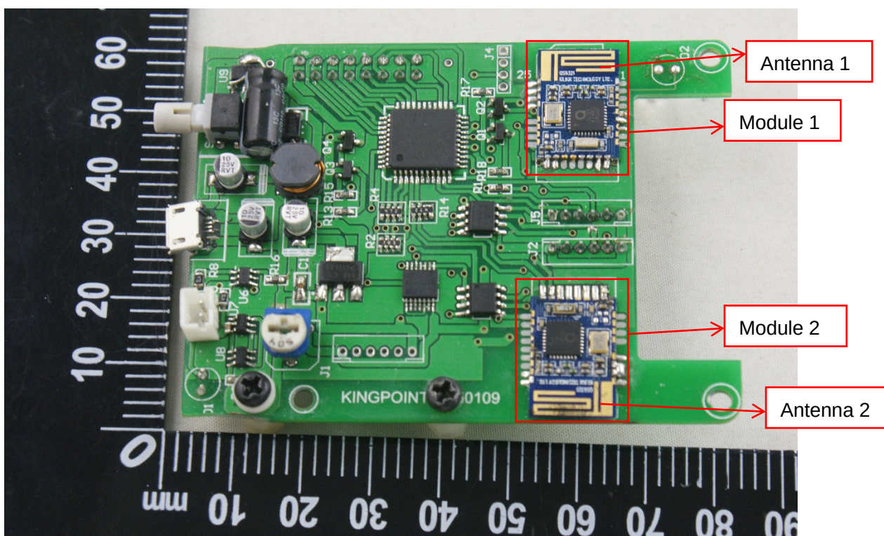
MAIN BOARD TOP VIEW 4
