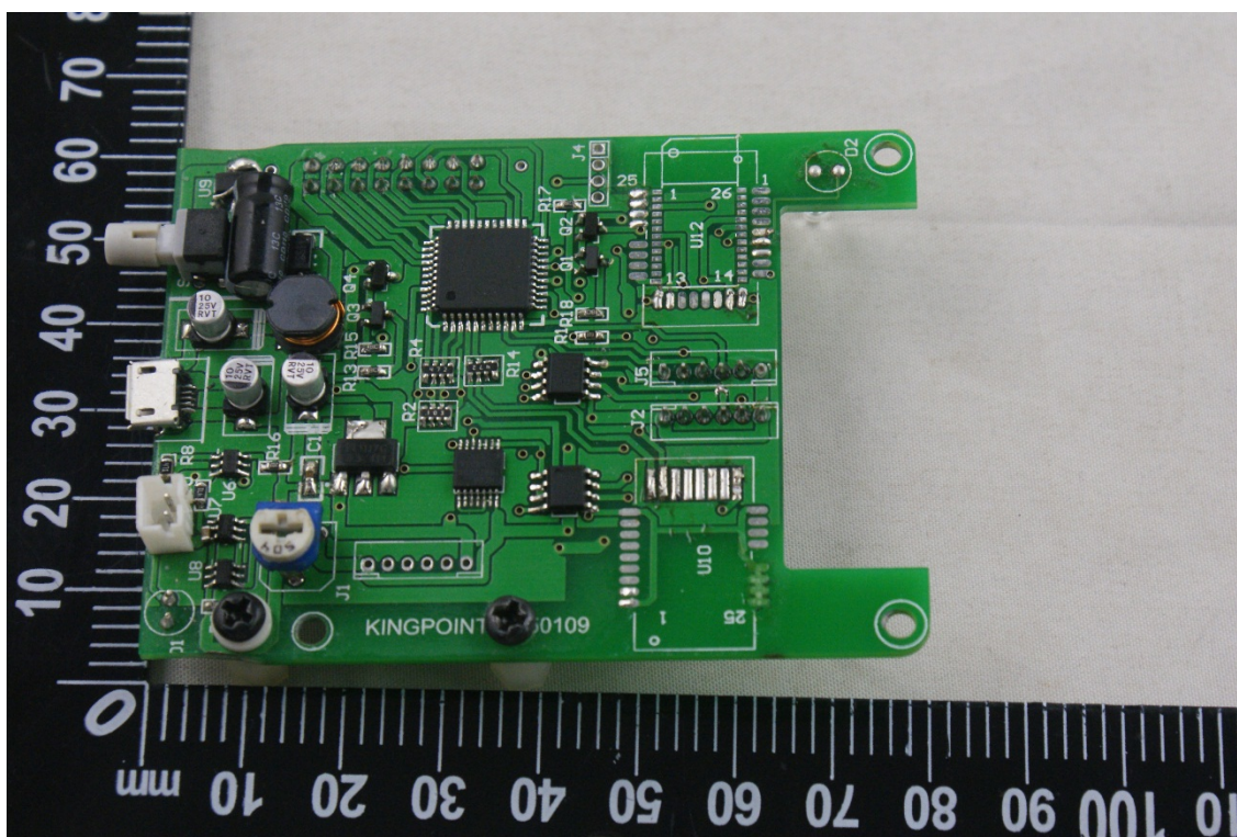
MAIN BOARD VIEW 5
