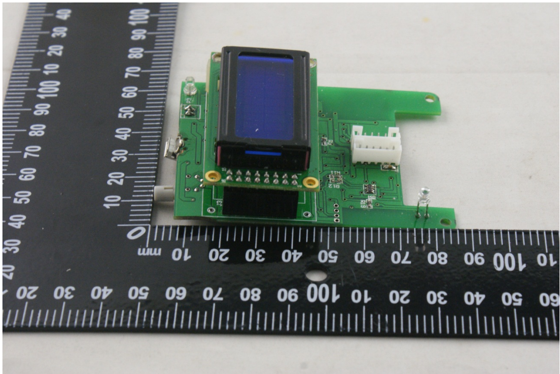
MAIN BOARD VIEW 2
