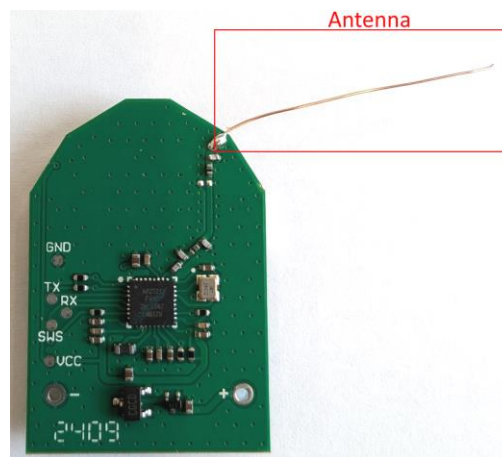
Figure 1: Antenna mounted on PCB
