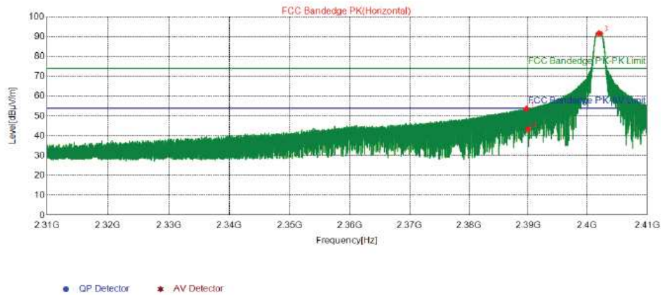
BLE_1M_2402_Ant1/ Horizontal-PK
