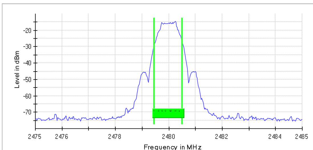
Mode 1 / CH39 (2480 MHz) 99 %Bandwidth
