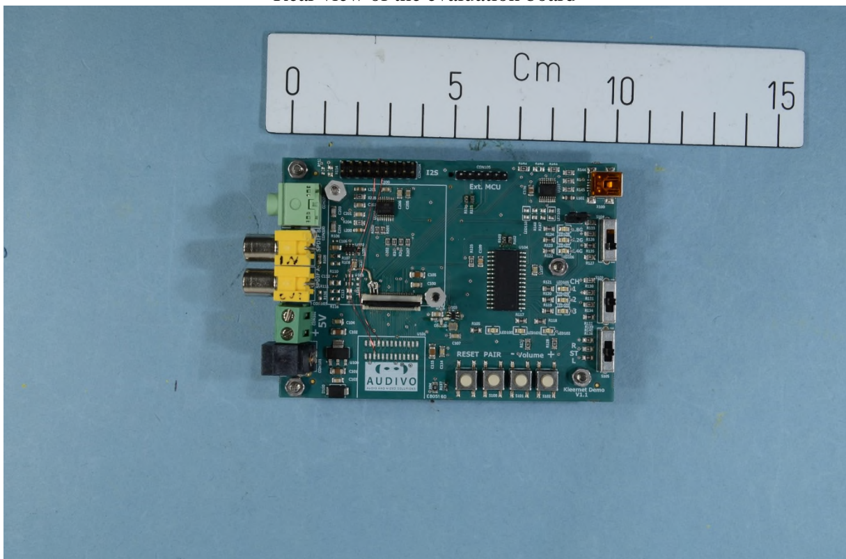
Front view of the evaluation board
