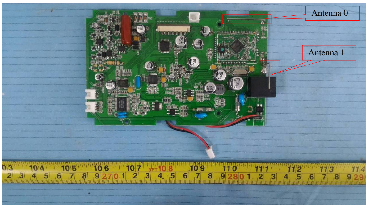
EU –Main Board 1 Top Shielding off View
