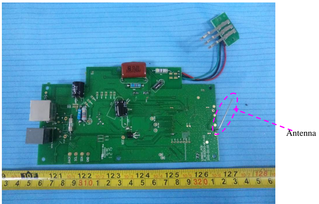
EUT (Base) –Main Board Bottom View
