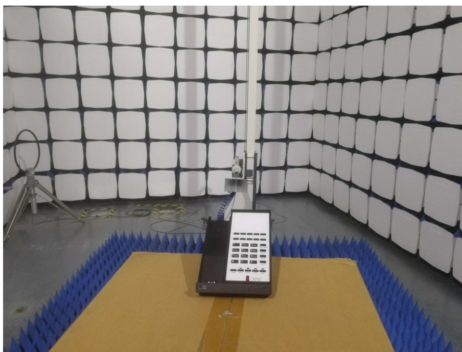
FP - Radiated Emission test view (Frequency above 1GHz)
