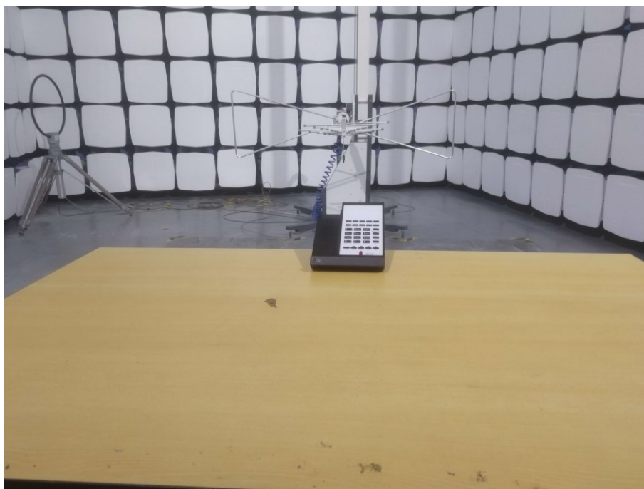
FP - Radiated Emission test view (Frequency from 30MHz to 1GHz)
