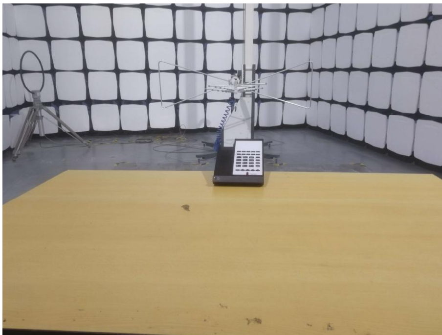
Radiated Emission test view (Frequency from 30MHz to 1GHz)
